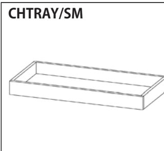
CHTRAY/SM Small Change Tray (with pad) w: 42" d: 17.25" h: 3.75"
